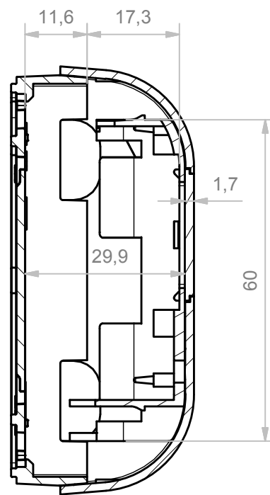
B-B (1:1)
